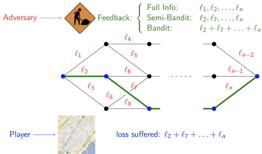
Figure 17.1: Path planning.
